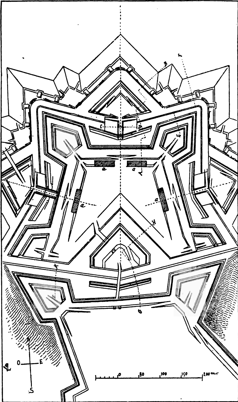
FIG. 66.—VAUBAN'S OUTWORK.
